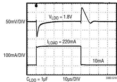
LD01 to LD03 Load Step Response
