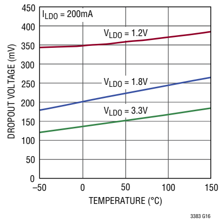
LD01 to LD03 Dropout Voltage vs Temperature
