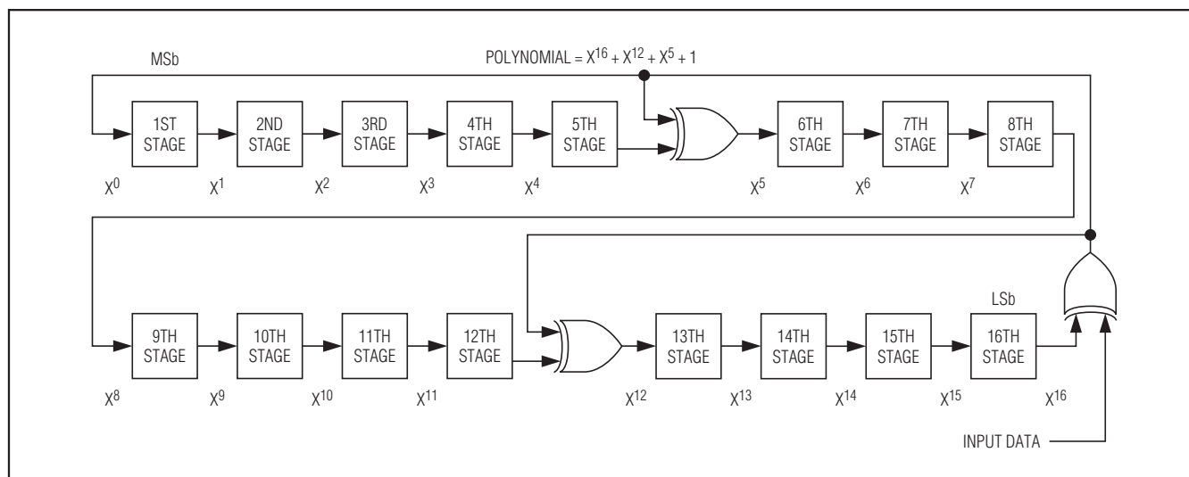
Figure 16. CRC-16-CCITT Generator
