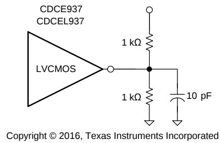
Figure 4. Test Load
