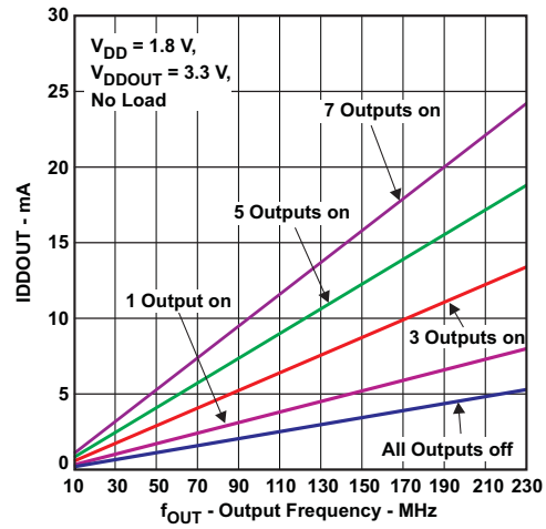
Figure 2. CDCE937 Output Current vs Output Frequency
