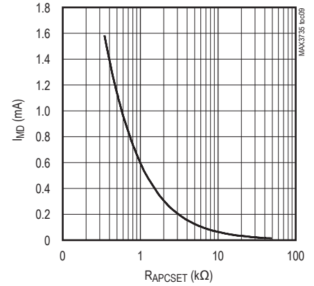
MONITOR DIODE CURRENT vs. R_{APCSET}
