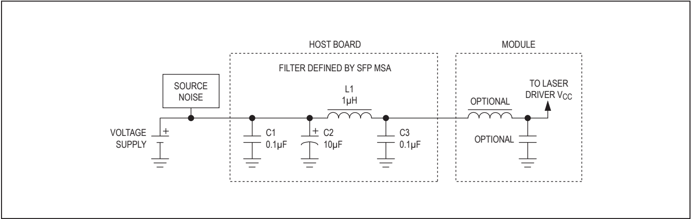
Figure 3. Supply Filter
