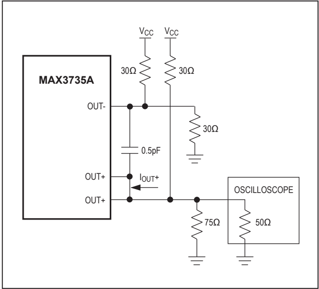
Figure 2. Output Termination for Characterization
