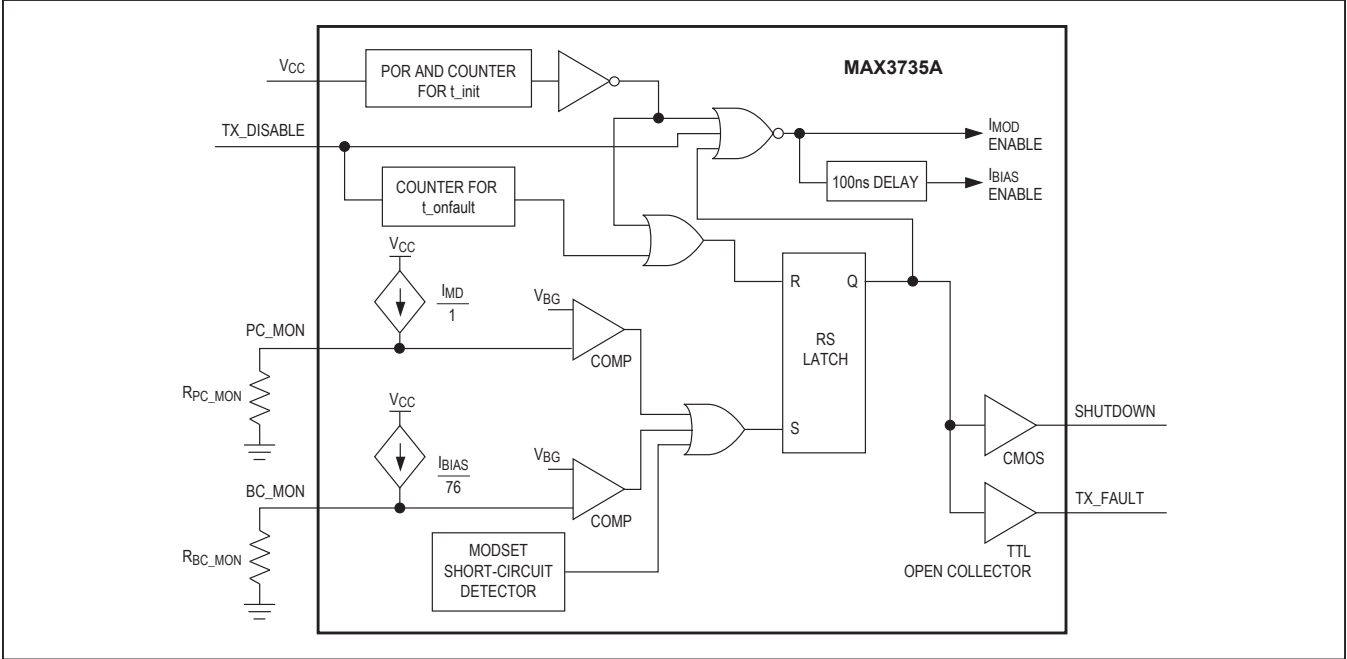
Figure 4. Safety Circuitry
