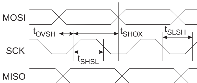
Figure 20-3. Serial Programming Timing
