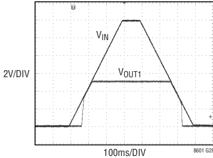
Channel 1 Start-Up and Dropout, R_L = 20\Omega
