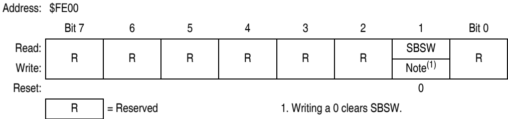
Figure 18-7. SIM Break Status Register (SBSR)
