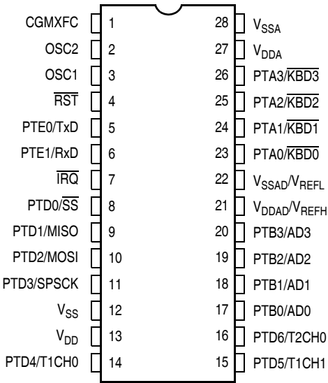
Figure 1-3. 28-Pin DIP and SOIC Pin Assignments
