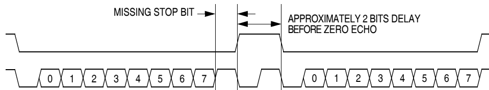
Figure 18-13. Break Transaction
