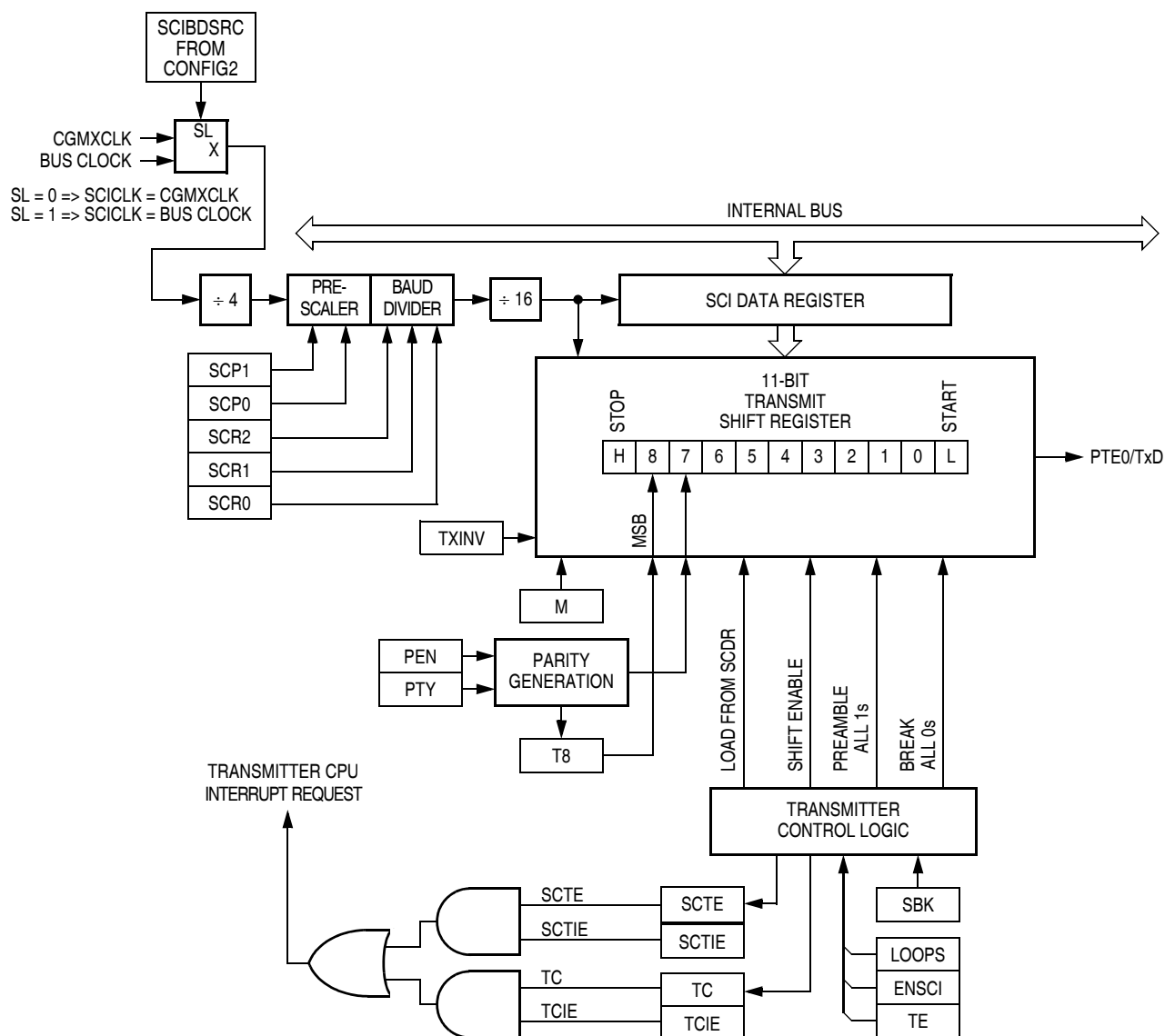
Figure 13-5. SCI Transmitter
