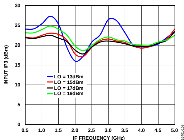
Figure 100. Input IP3 vs. IF Frequency at Various LO Power Levels, T_A = 25^\circ\text{C}
