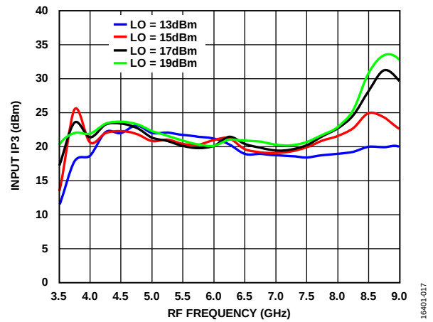
Figure 17. Input IP3 vs. RF Frequency at Various LO Power Levels, TA = 25°C
