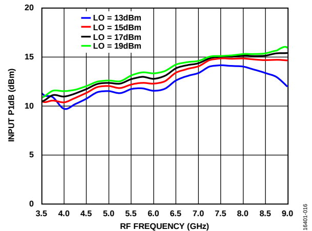
Figure 19. Input P1dB vs. RF Frequency at Various LO Power Levels, TA = 25°C
