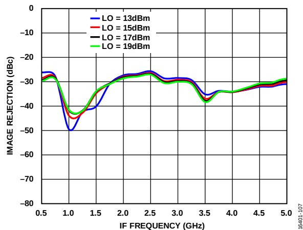
Figure 99. Image Rejection vs. IF Frequency at Various LO Power Levels, T_A = 25^\circ\text{C}
