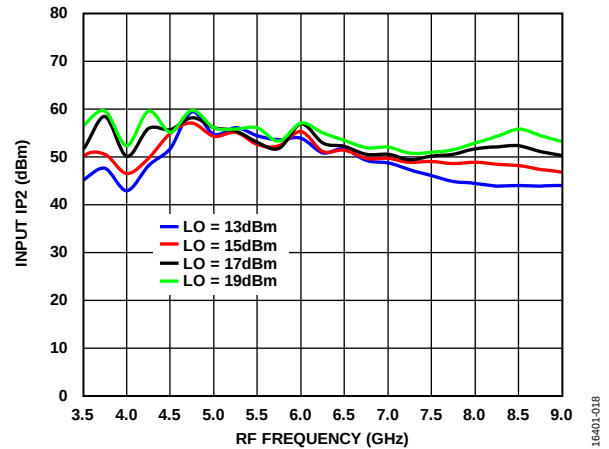
Figure 18. Input IP2 vs. RF Frequency at Various LO Power Levels, TA = 25°C
