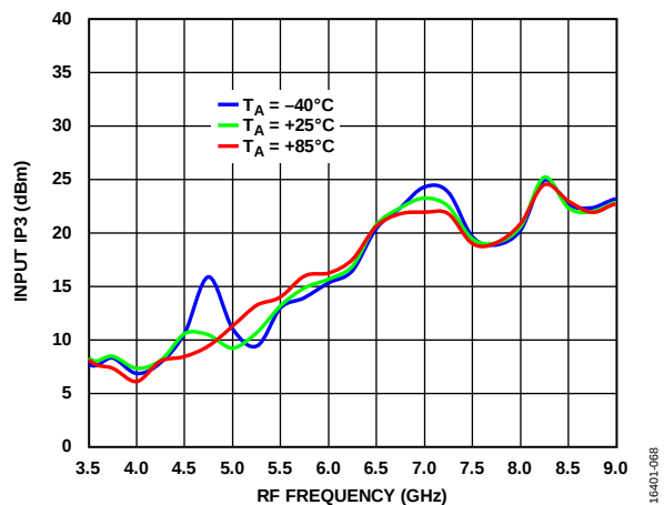
Figure 61. Input IP3 vs. RF Frequency at Various Temperatures, LO = 15 dBm
