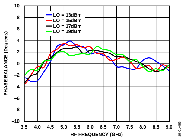
Figure 75. Phase Balance vs. RF Frequency at Various LO Power Levels, T_A = 25^\circ\text{C}
