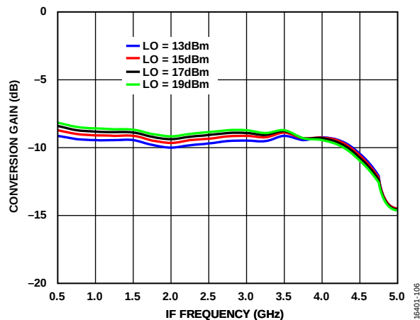
Figure 98. Conversion Gain vs. IF Frequency at Various LO Power Levels, T_A = 25^\circ\text{C}
