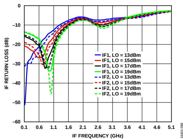
Figure 88. IF Return Loss vs. IF Frequency at Various LO Power Levels, LO = 5 GHz, T_A = 25^\circ\text{C}
