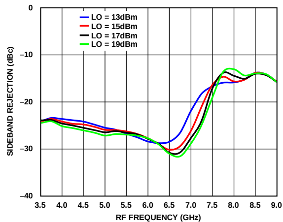
Figure 71. Sideband Rejection vs. RF Frequency at Various LO Power Levels, T_A = 25^\circ\text{C}
