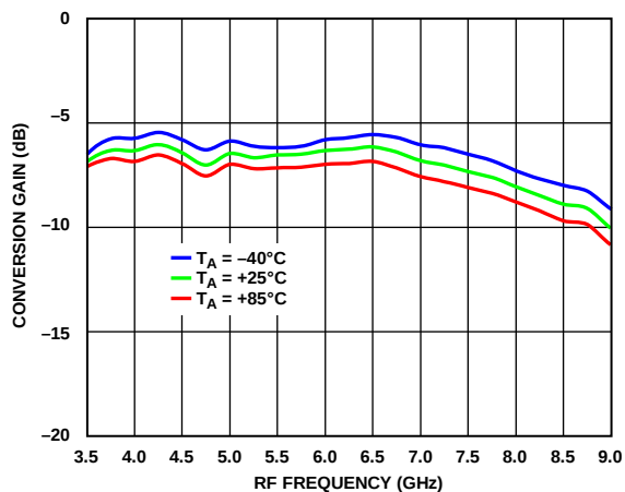
Figure 52. Conversion Gain vs. RF Frequency at Various Temperatures, LO = 15\text{ dBm}
