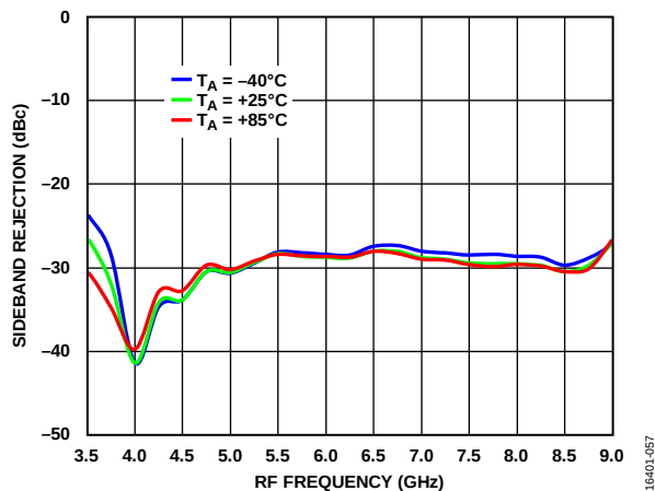
Figure 53. Sideband Rejection vs. RF Frequency at Various Temperatures, LO = 15\text{ dBm}
