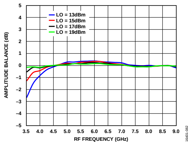
Figure 74. Amplitude Balance vs. RF Frequency at Various LO Power Levels, T_A = 25^\circ\text{C}
