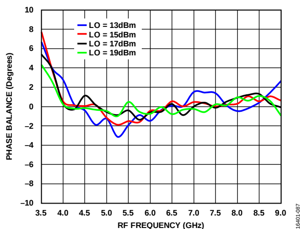
Figure 79. Phase Balance vs. RF Frequency at Various LO Power Levels, TA = 25°C
