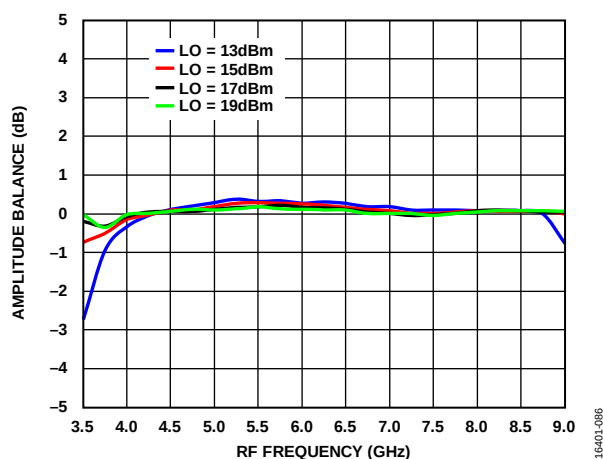
Figure 78. Amplitude Balance vs. RF Frequency at Various LO Power Levels, TA = 25°C
