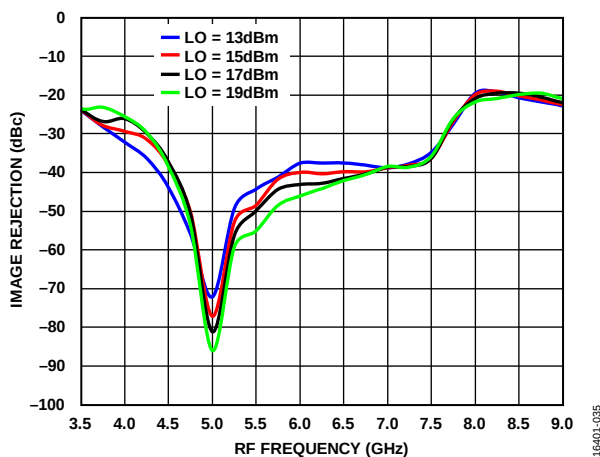
Figure 37. Image Rejection vs. RF Frequency at Various LO Power Levels, T_A = 25^\circ\text{C}
