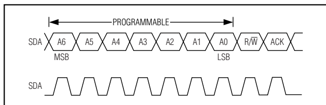
Figure 6. Slave Address
