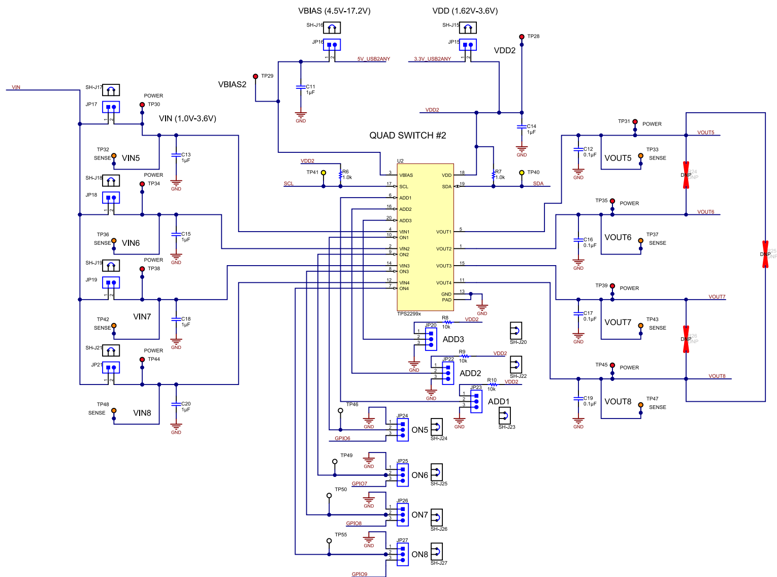
Figure 25. I²C Load Switch EVM Board Schematic (1 of 3)
