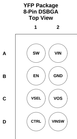
Pin Functions TPS62746
