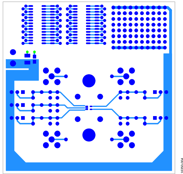
Figure 4. EVAL-5SC70EBZ Evaluation Board Top Layer
