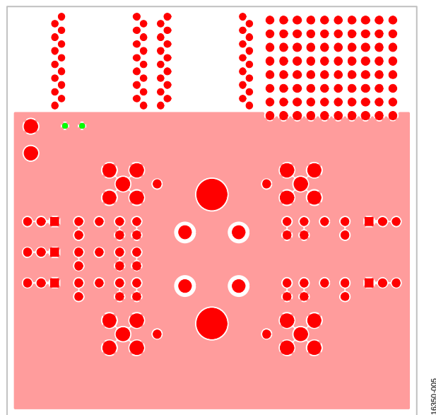
Figure 5. EVAL-5SC70EBZ Evaluation Board Bottom Layer
