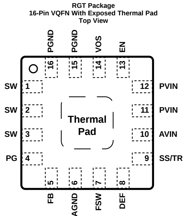
Pin Functions
