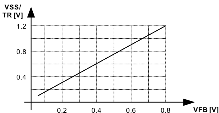
Figure 25. Voltage Tracking Relationship
