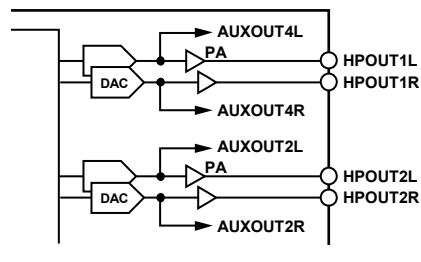
Figure 30. Headphone Outputs Section
