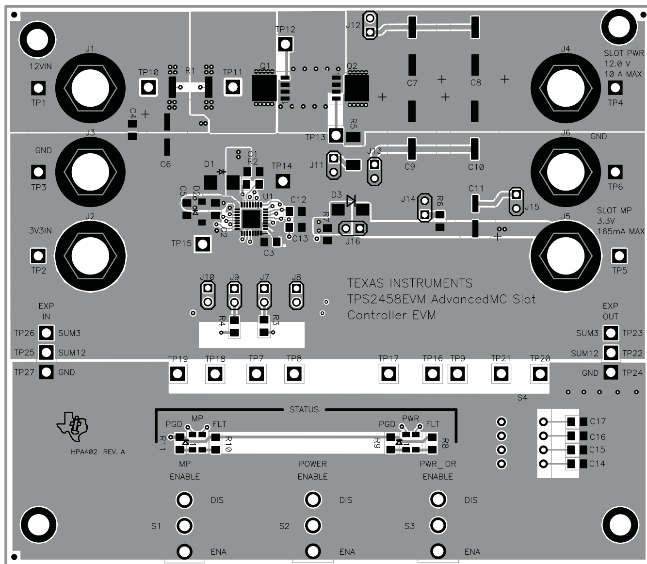
Figure 5. Top Assembly
