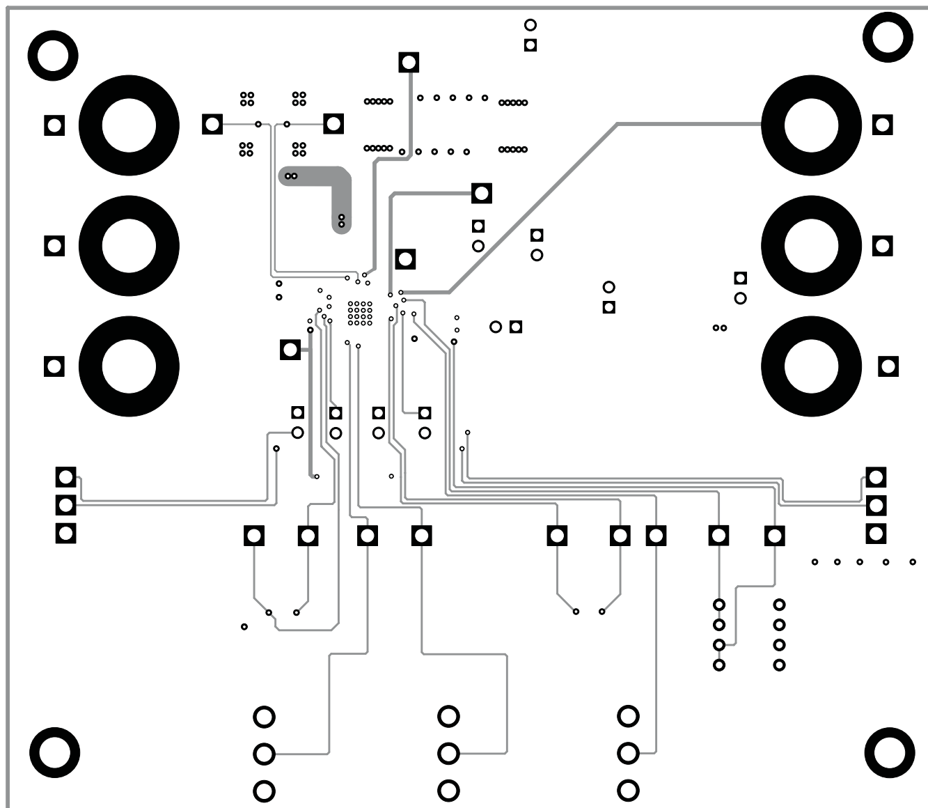
Figure 8. Layer 3 Routing
