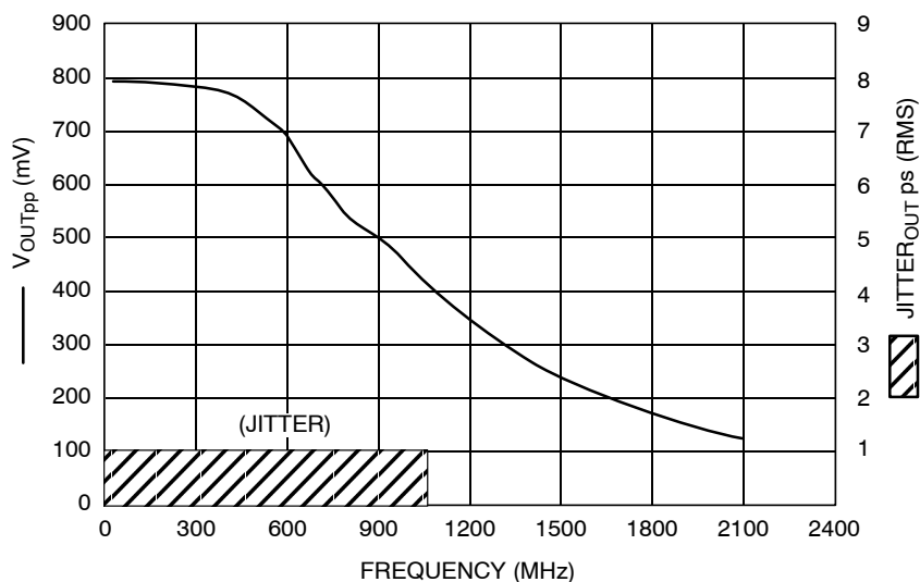
Figure 2. F_{\max} /Jitter
