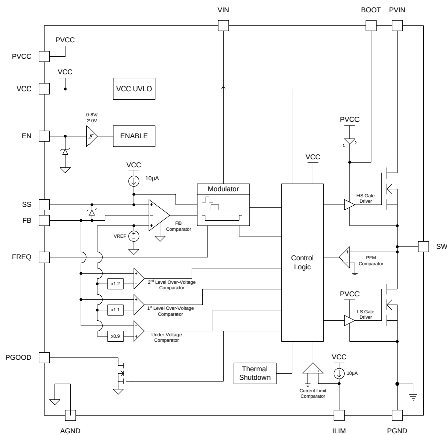
Figure 2. Block Diagram
