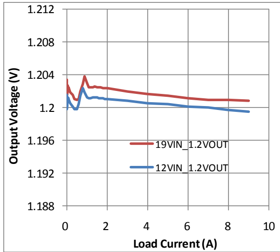
Figure 11. Load Regulation
