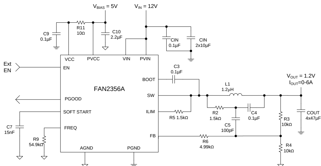
Figure 1. Typical Application
