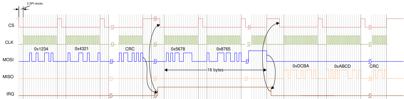
Figure 5-11. SPI Communication
