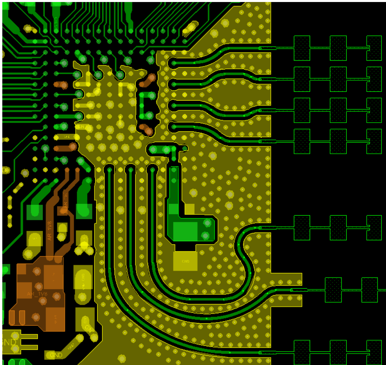
Figure 7-4. Top Layer Routing Closeup
