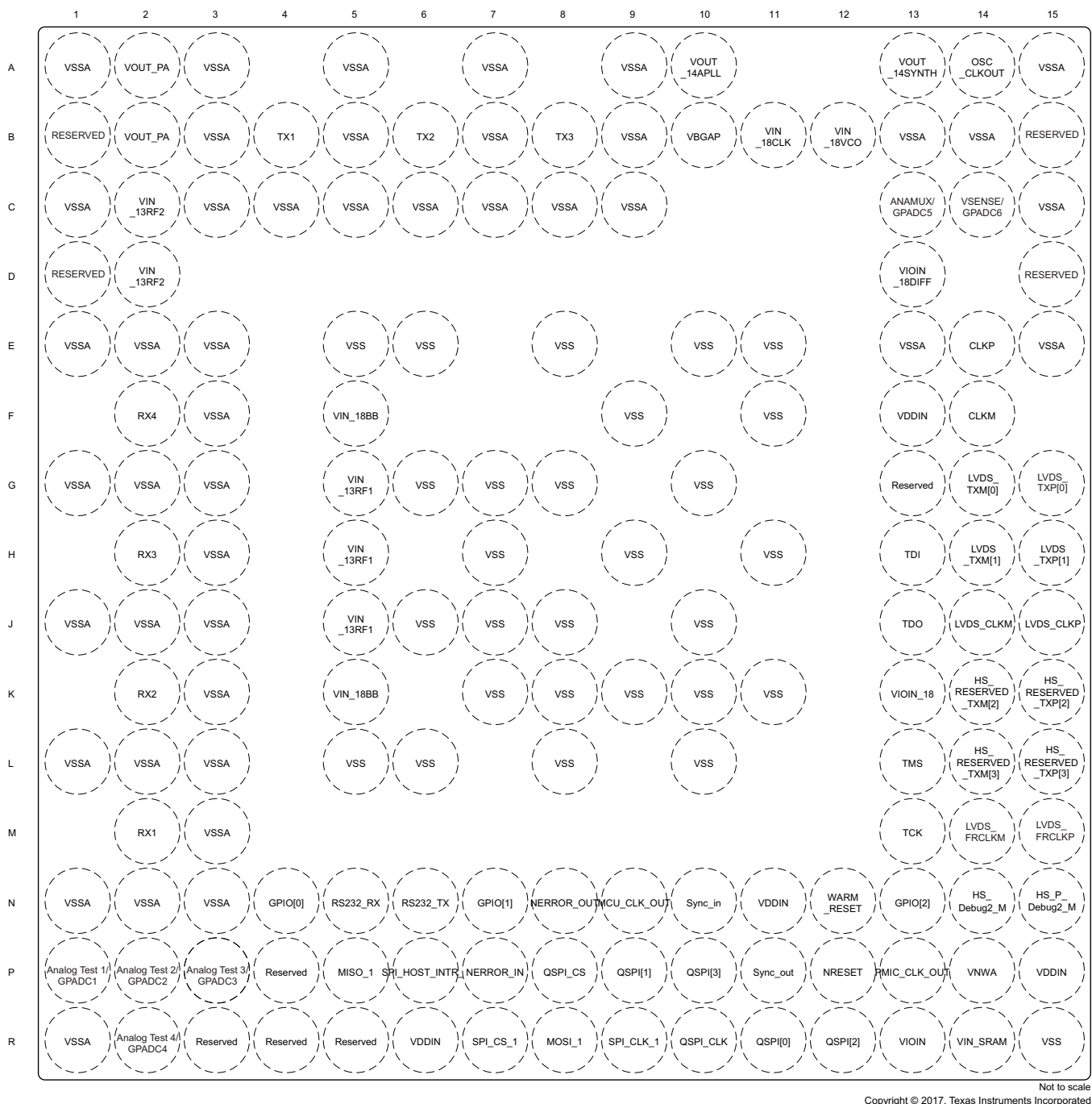
Figure 4-1. Pin Diagram
