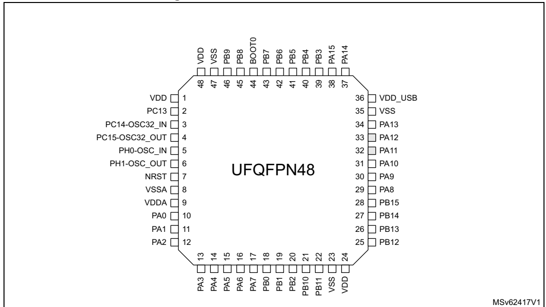
Figure 4. STM32L082xx UFQFPN48
