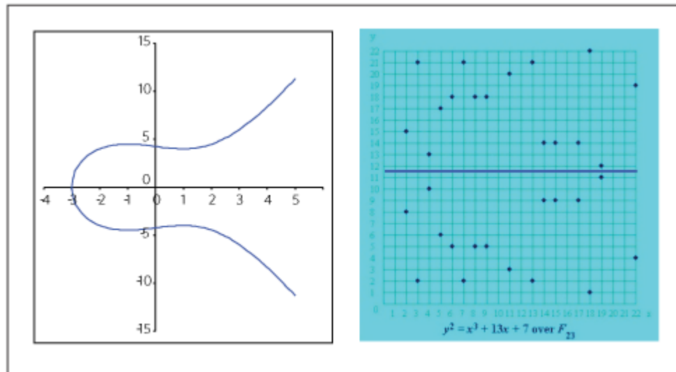
Figure 1. Third-degree elliptic curves, real domain (left), over prime field (right).
