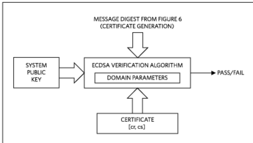
Figure 8. Verifying the authenticator's public key using the certificate.
