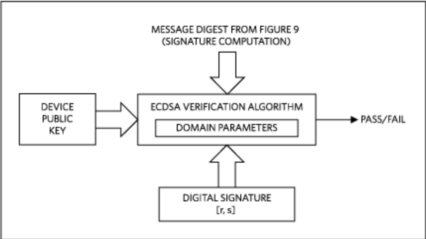
Figure 10. Verifying the signature computed by the authenticator.
