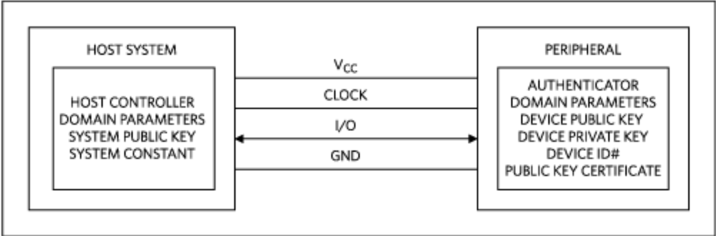
Figure 5. Hardware configuration of an ECDSA authentication system.
