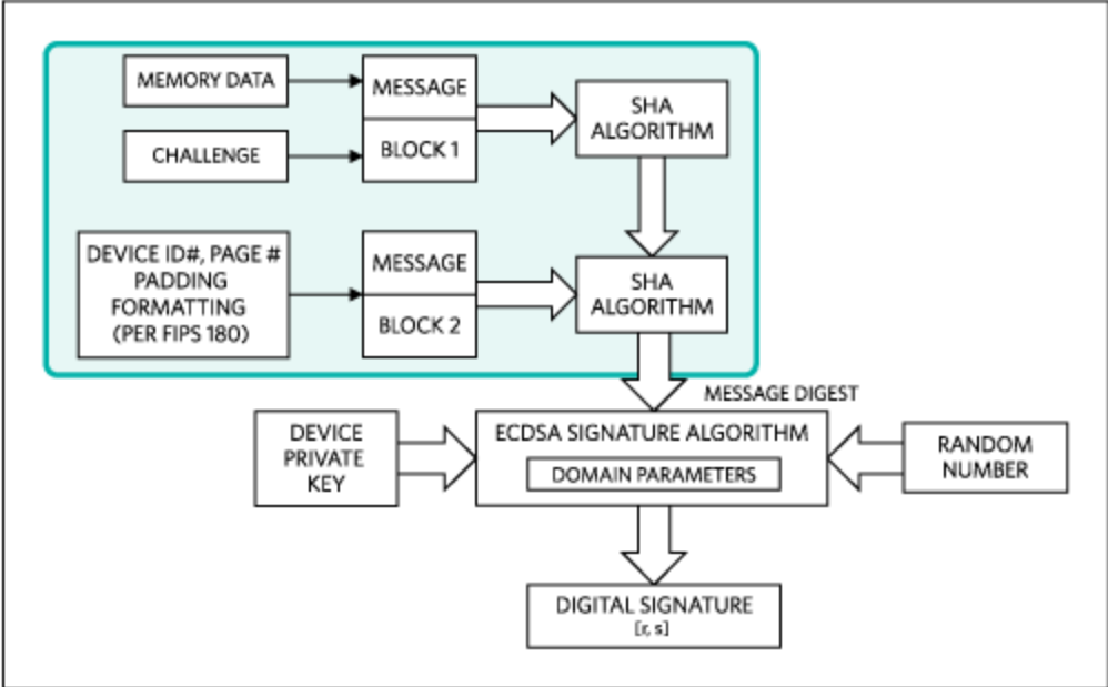
Figure 9. Signature computation performed by the authenticator.
