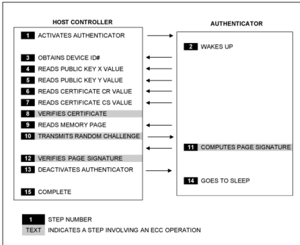
Figure 7. Typical transaction flow to authenticate a deployed peripheral.
