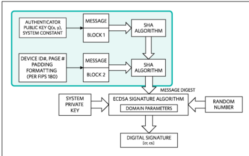
Figure 6. Certificate generation by a key-management system.
