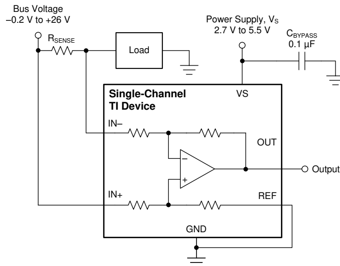
Figure 44. Unidirectional Application
