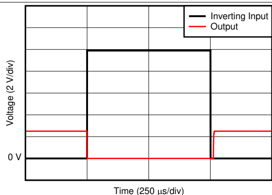
Figure 31. Step Response
