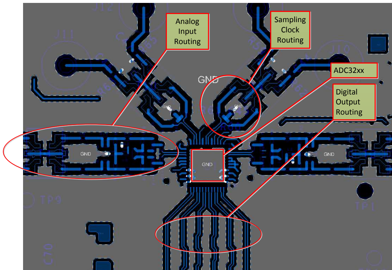
Figure 181. Typical Layout of the ADC322x Board
