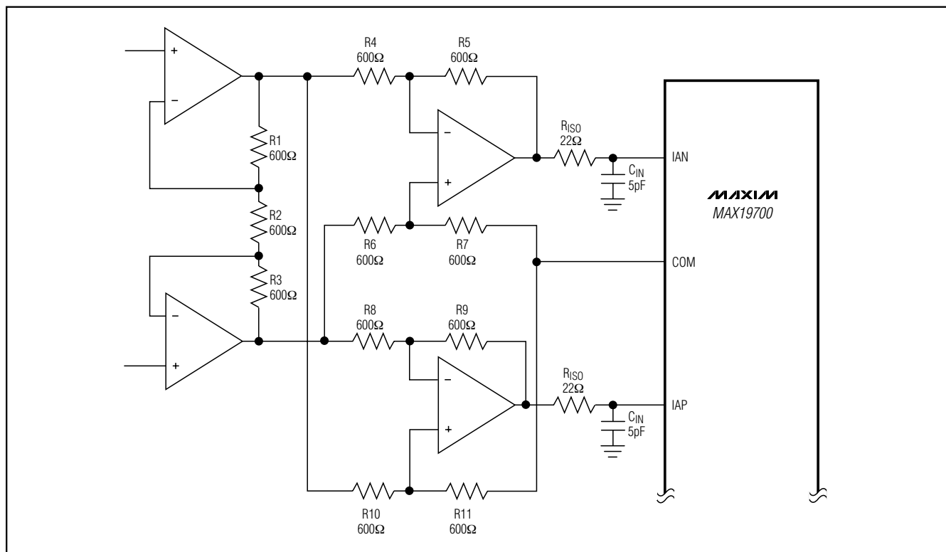
Figure 11. Rx ADC DC-Coupled Differential Drive
