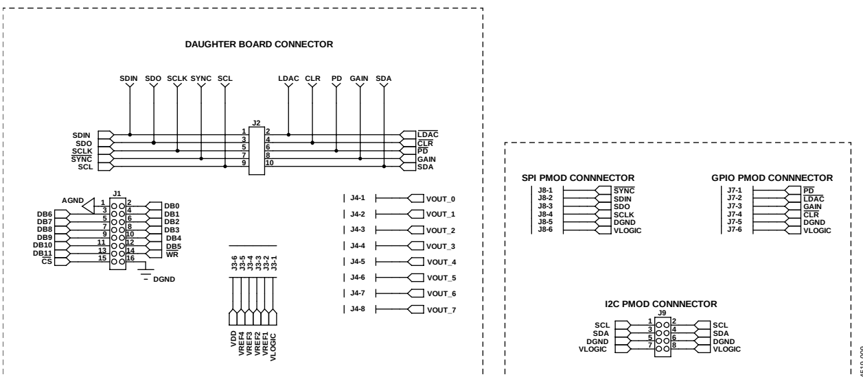
Figure 9. EVAL-MBnanoDAC-SDZ Motherboard Connectors to Daughter Board and Serial Interface
