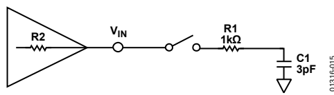
Figure 10. Equivalent Sampling Circuit
