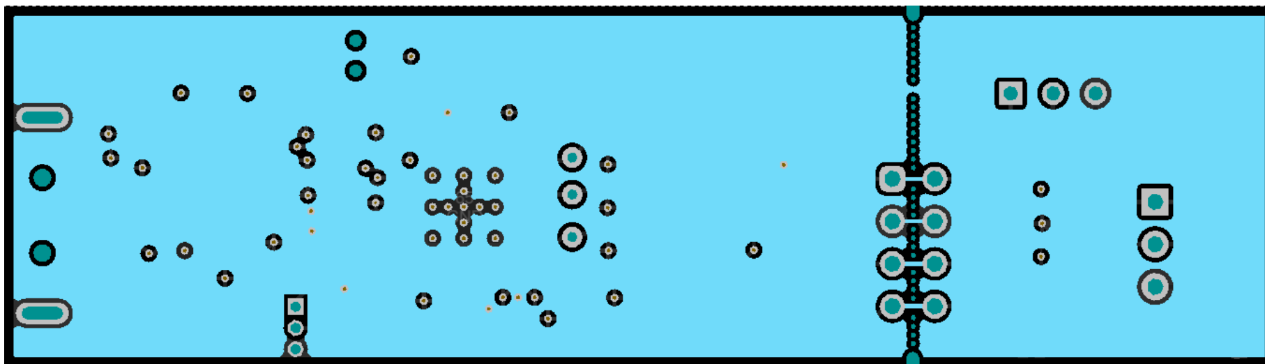
Figure 22. Power Layer
