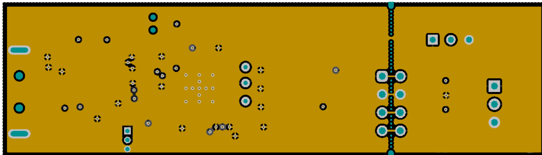
Figure 21. Ground Layer
