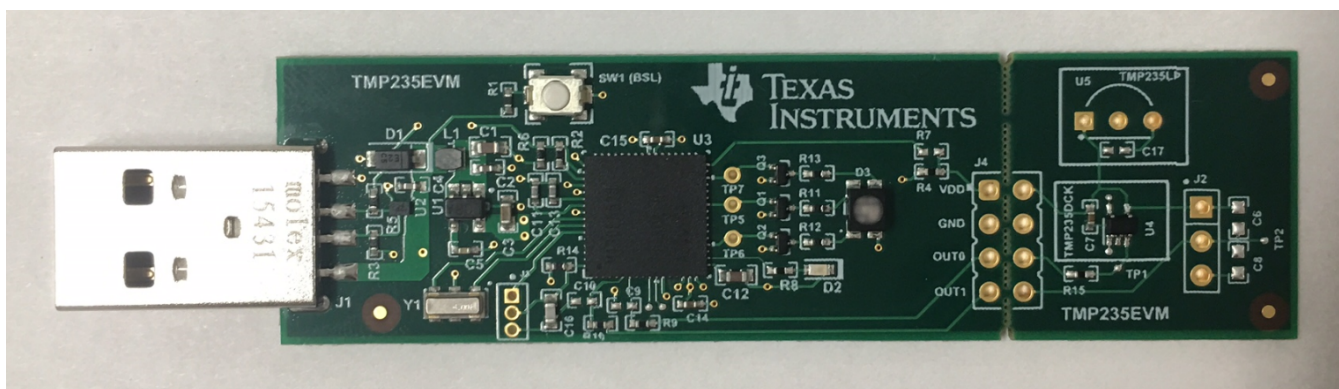
Figure 1. TMP235EVM Top View
