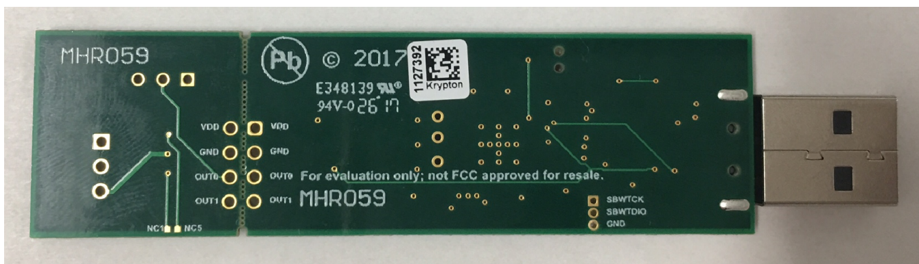
Figure 2. TMP235EVM Bottom View
