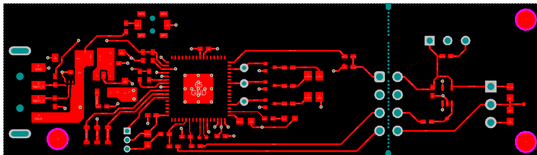
Figure 20. Top Signal Layer
