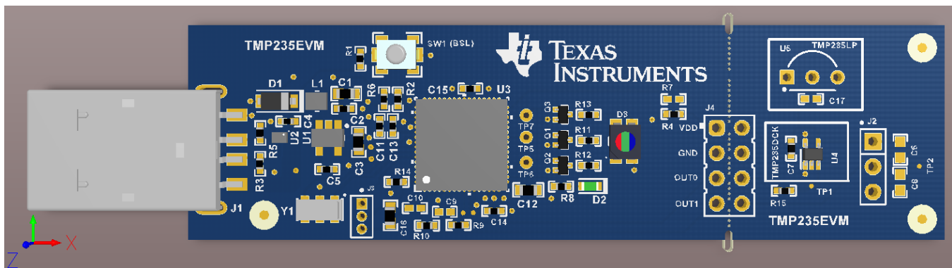
Figure 6. EVM 3D Top View
