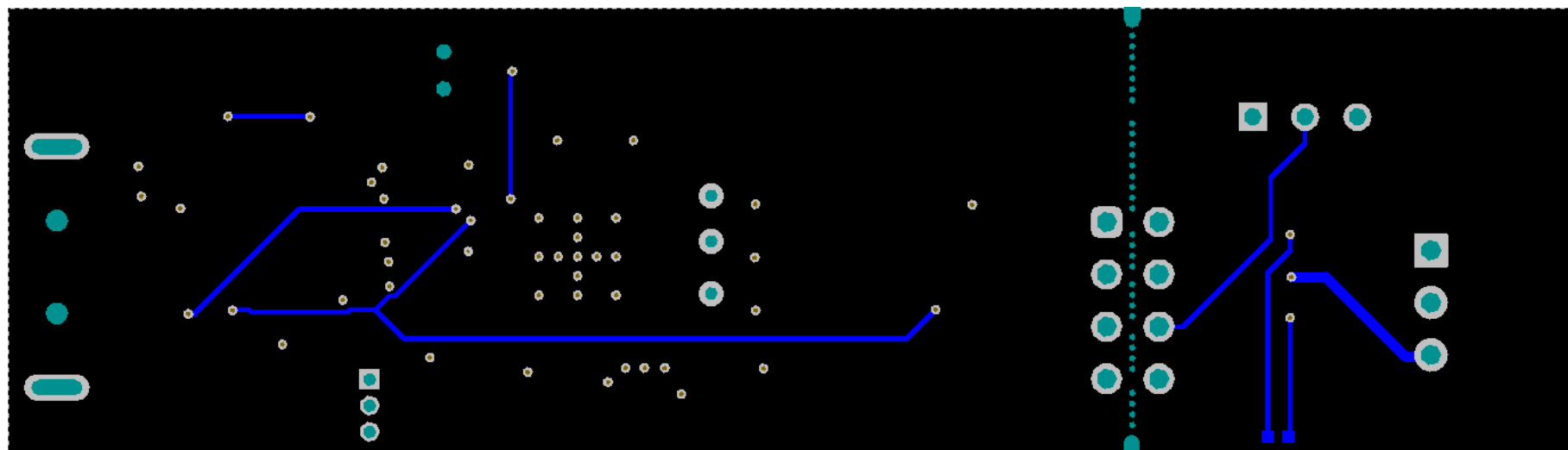
Figure 23. Bottom Signal Layer
