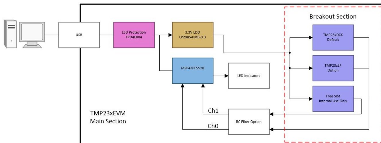
Figure 4. EVM Block Diagram
