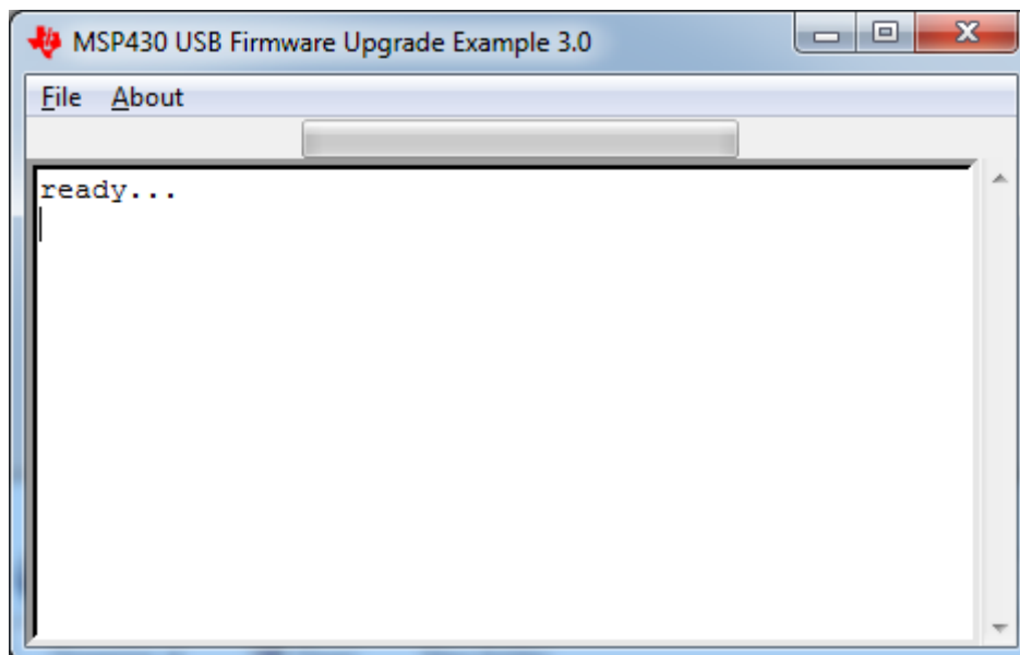
Figure 16. BSL Ready
