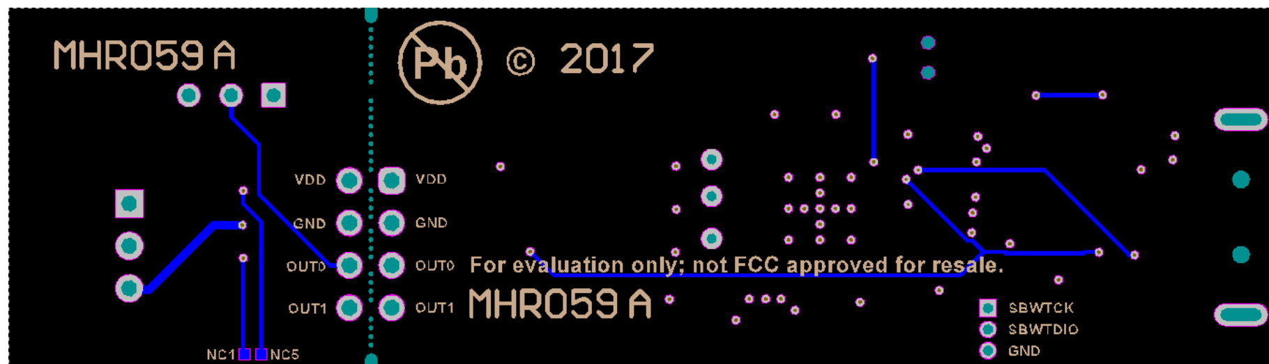
Figure 24. Bottom Layers
