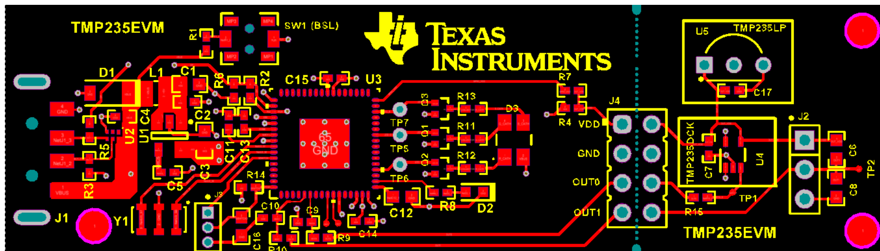
Figure 19. Top Layers
