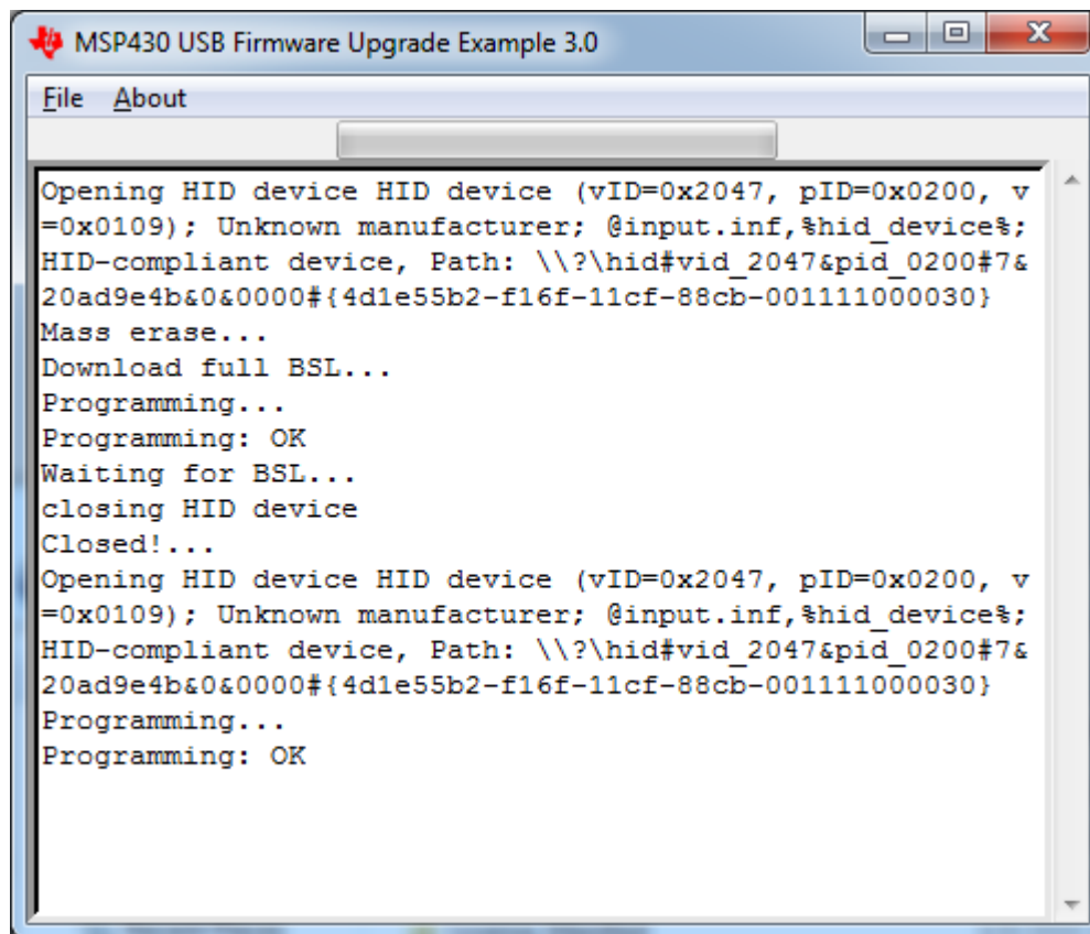
Figure 17. FW Upload Success
