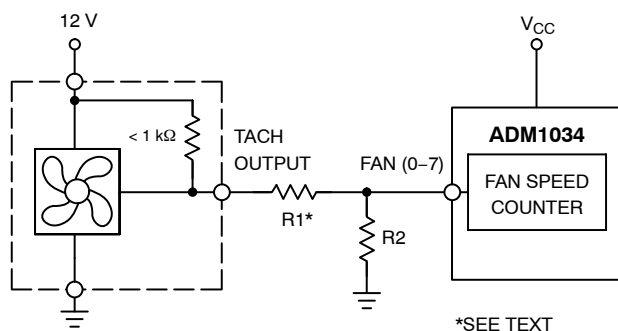
Figure 38. Fan with Strong TACH. Pullup to >V_{\text{CC}} or Totem-Pole Output, Attenuated with R1/R2
