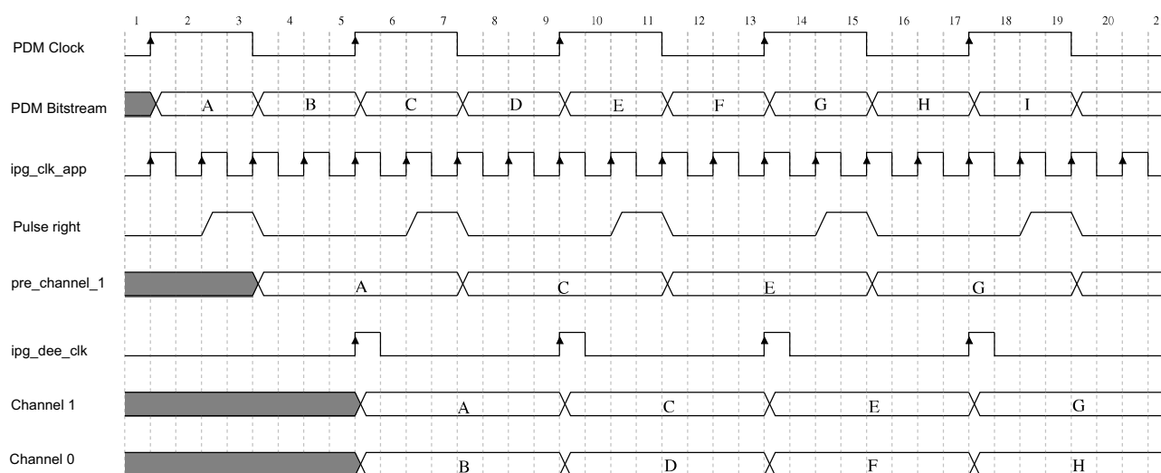
Figure 32. PDM input timing
