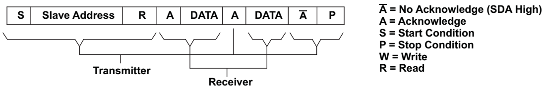
Figure 76. I²C Read Cycle
