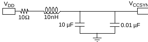
Figure 34. V_{CCSYN} Bypass
