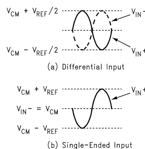
Figure 30. Expected Input Signal Range
