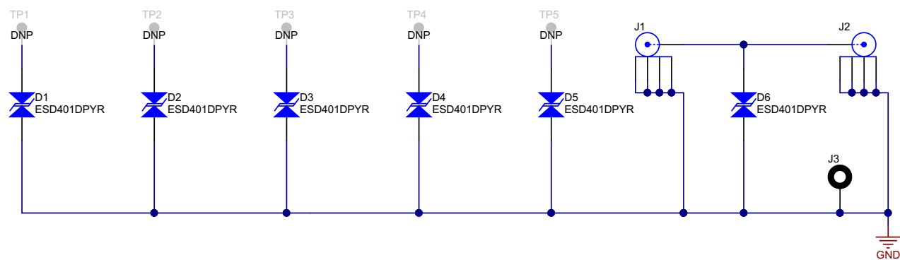
Figure 4. ESD401EVM Schematic
