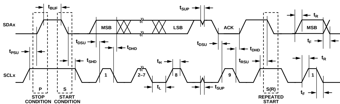
Figure 2. I 2 C-Compatible Interface Timing
