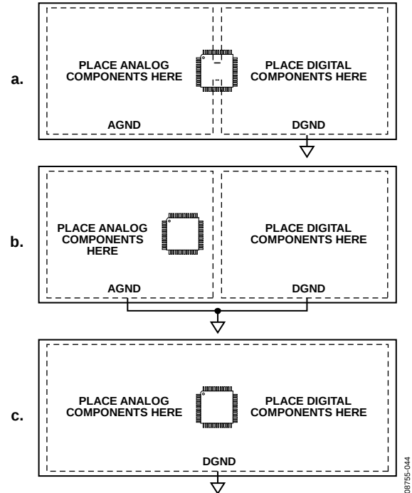
Figure 43. System Grounding Schemes
