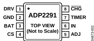
Figure 2. 8-Lead MSOP Pin Configuration
