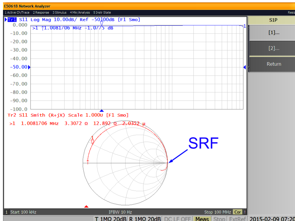
Figure 20. Measurement of SRF with a VNA
