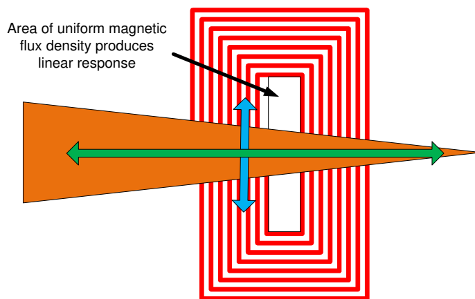
Figure 5. Rectangular Coil is Insensitive to a Y-axis Shift
