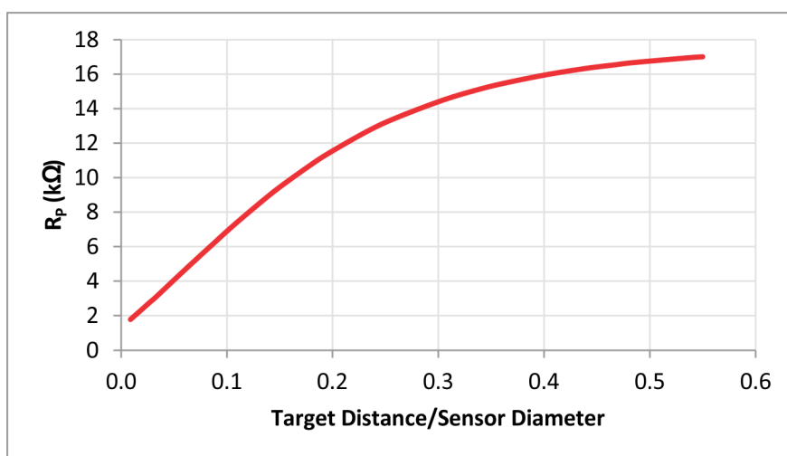
Figure 15. R_p Versus Normalized Target Distance
