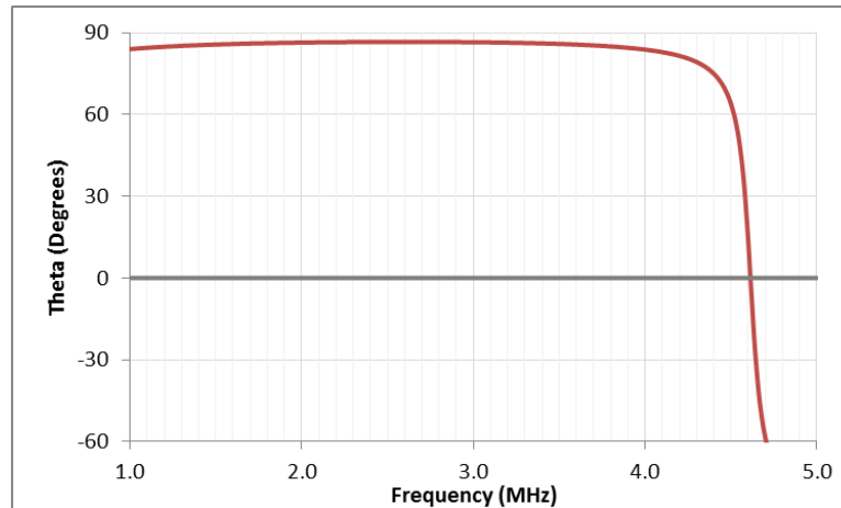
Figure 19. Inductance T Versus Frequency
