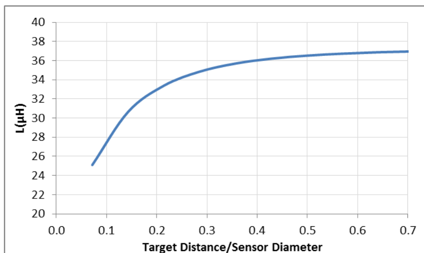
Figure 16. Inductance Versus Normalized Target Distance
