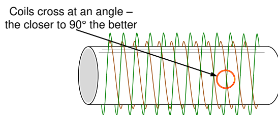
Figure 23. Winding Crossing for Honeycomb Coil
