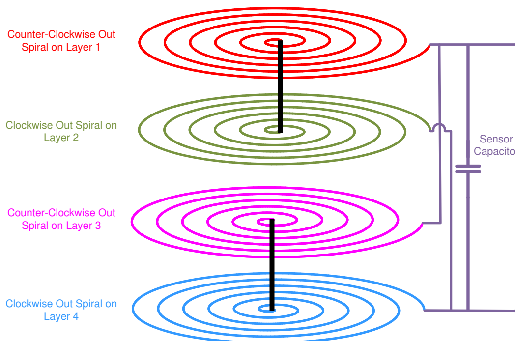
Figure 14. Multi-layer Parallel Inductor
