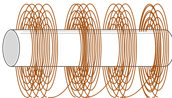
Figure 24. Combination of Both Winding-out and Crossing
