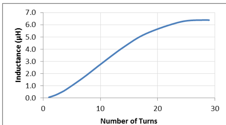
Figure 9. Inductance Versus Number of Turns for 18-mm Circular Inductor
