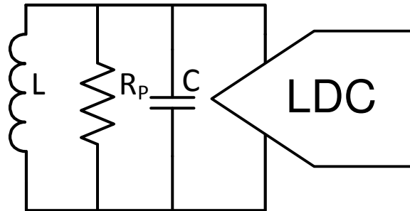
Figure 3. RLC Model
