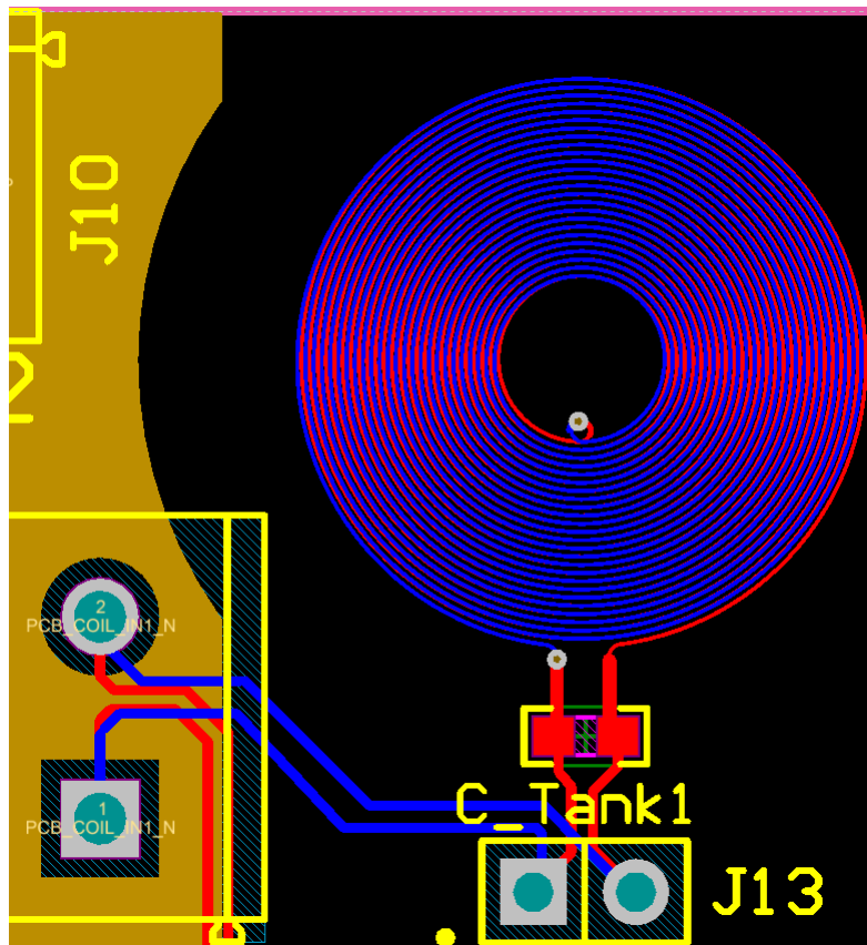
Figure 26. Minimize Copper Around the Sensor
