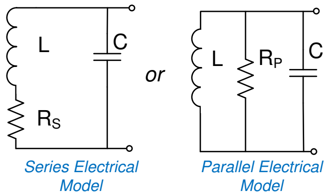
Figure 2. R_s and R_p
