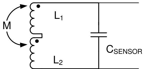
Figure 12. Mutual Inductance for Two-Layer Sensor (Ignoring R_p )
