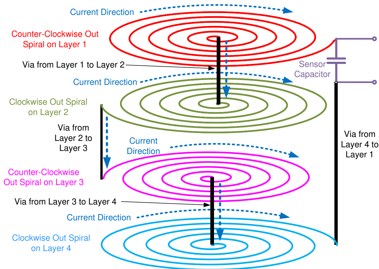
Figure 10. Multiple Layer Inductor Construction (Series)
