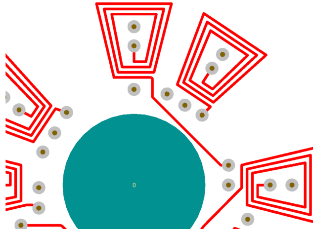
Figure 6. Trapezoidal Inductor for Rotational Encoding
