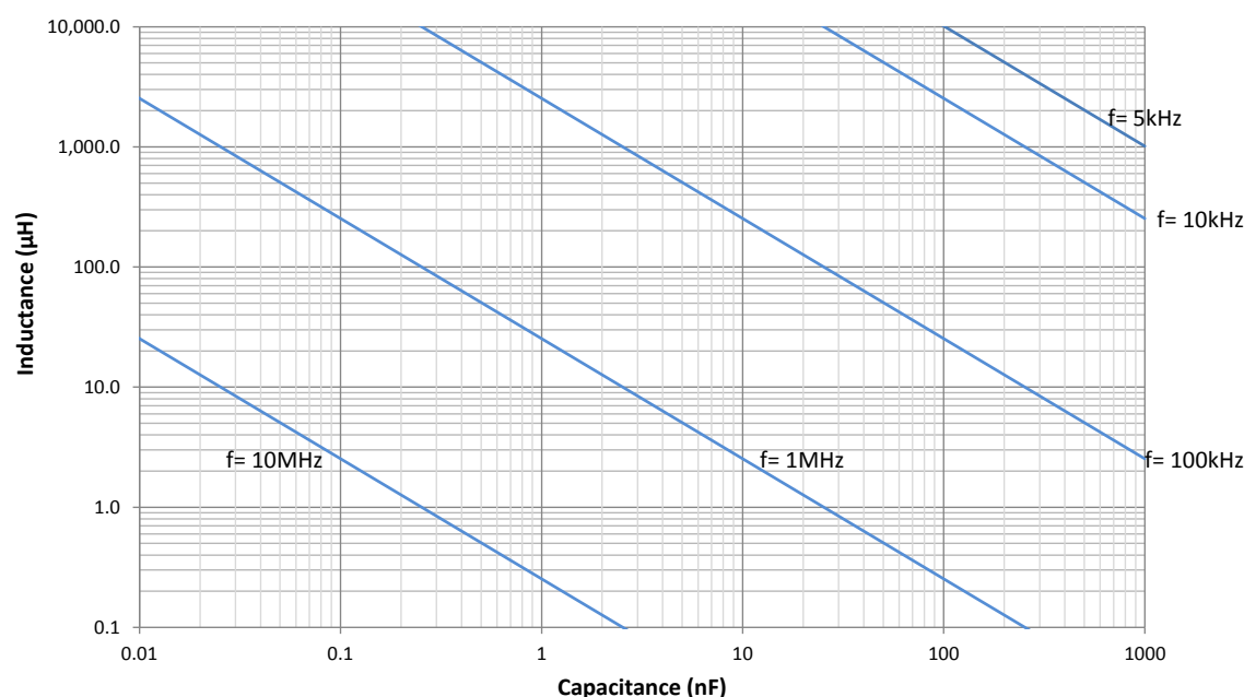
Figure 1. Sensor Frequency Versus Inductance and Capacitance
