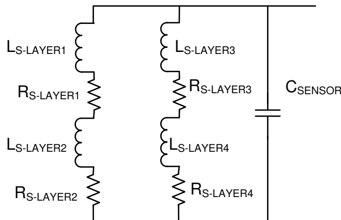
Figure 13. Multi-layer Parallel Coil Schematic
