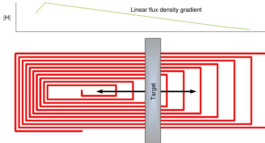
Figure 7. "Stretched" Rectangular Coil for lateral Position Measurement
