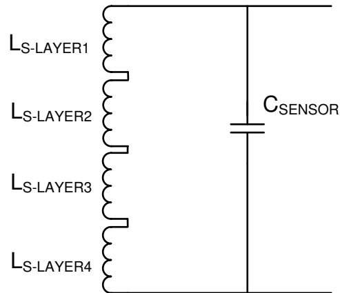
Figure 11. Simplified Electrical Model of Four-Layer Series Sensor (Ignoring R_p )
