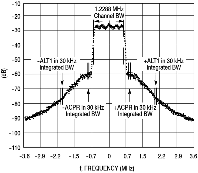
Figure 26. Single-Carrier N-CDMA Spectrum
