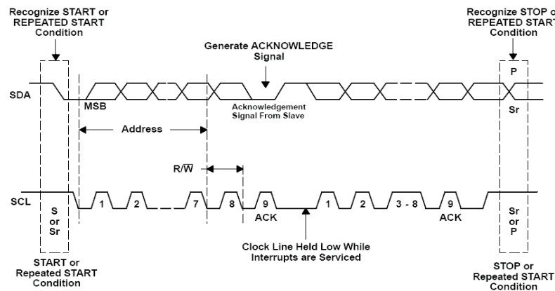
Figure 38. Bus Protocol
