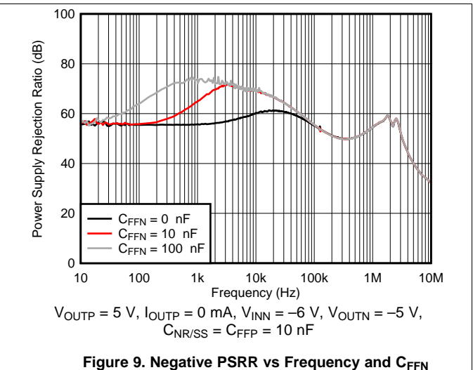
Figure 9. Negative PSRR vs Frequency and C_{FFN}
