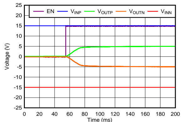
Monotonic Start-Up Tracking
