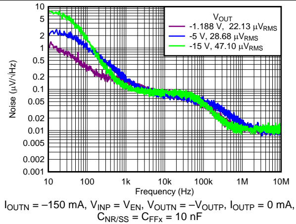
Figure 15. Negative Spectral Noise Density vs Frequency and V_{OUTN}
