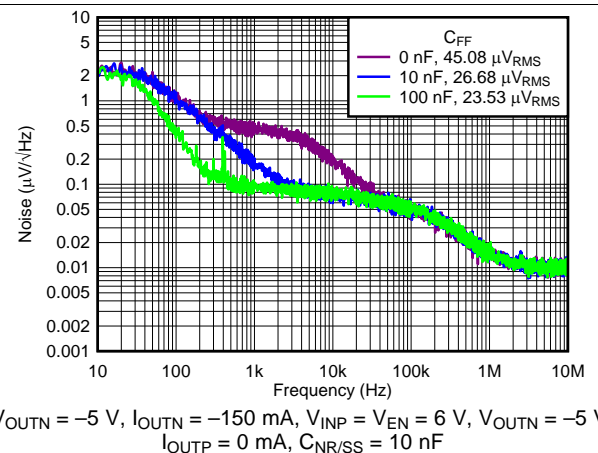
Figure 19. Negative Spectral Noise Density vs Frequency and C_{FF}
