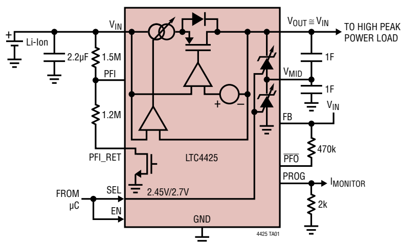
Charging 2-Cell Series Supercapacitor from Li-Ion Source
