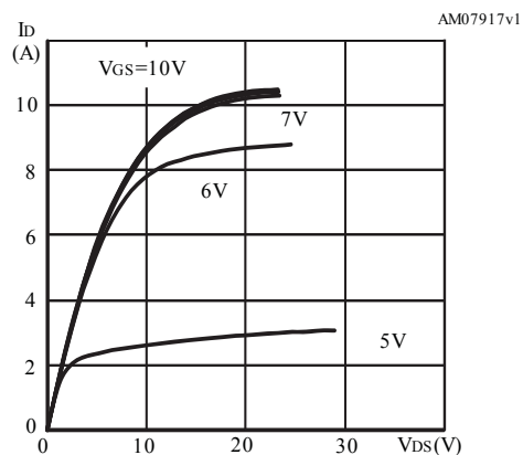
Figure 5. Output characteristics
