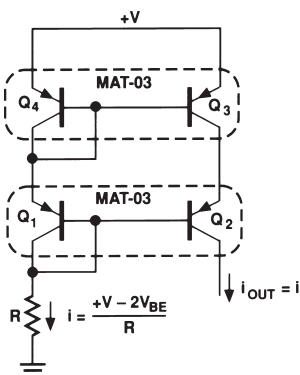
Figure 5. Cascode Current Source
