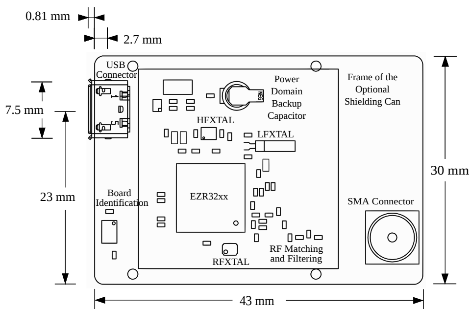
Figure 5.1. BRD4502D (Rev. A00) top view
