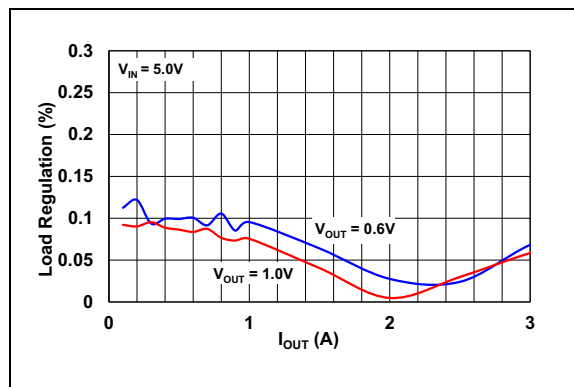
FIGURE 2-10: Load Regulation: V_{OUT} Voltage Variation vs. I_{OUT} .
