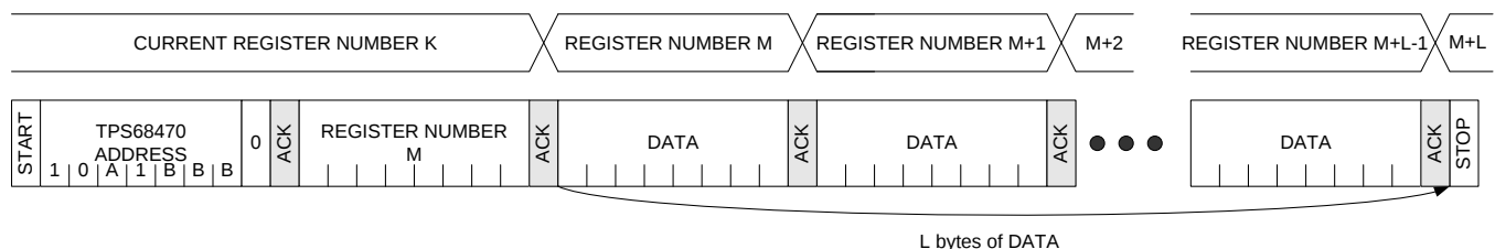
Figure 12. Sequential Write
