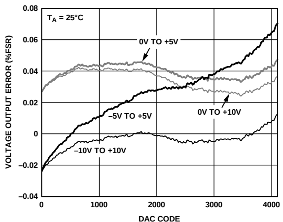
Figure 2. Voltage Output Error
