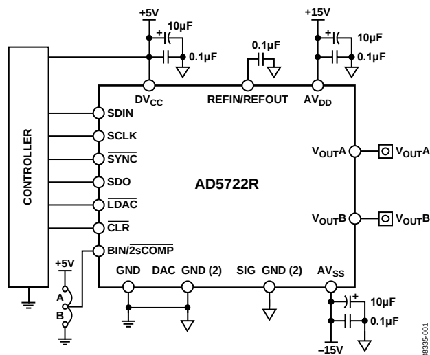
Figure 1. Unipolar/Bipolar Configuration for the AD5722R DAC
