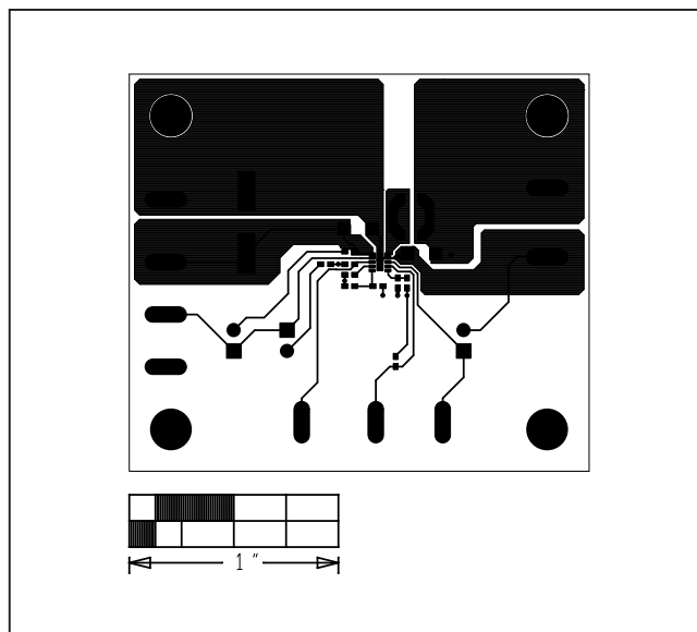
Figure 3. MAX17552 5V EV Kit (TDFN) PCB Layout—Component Side
