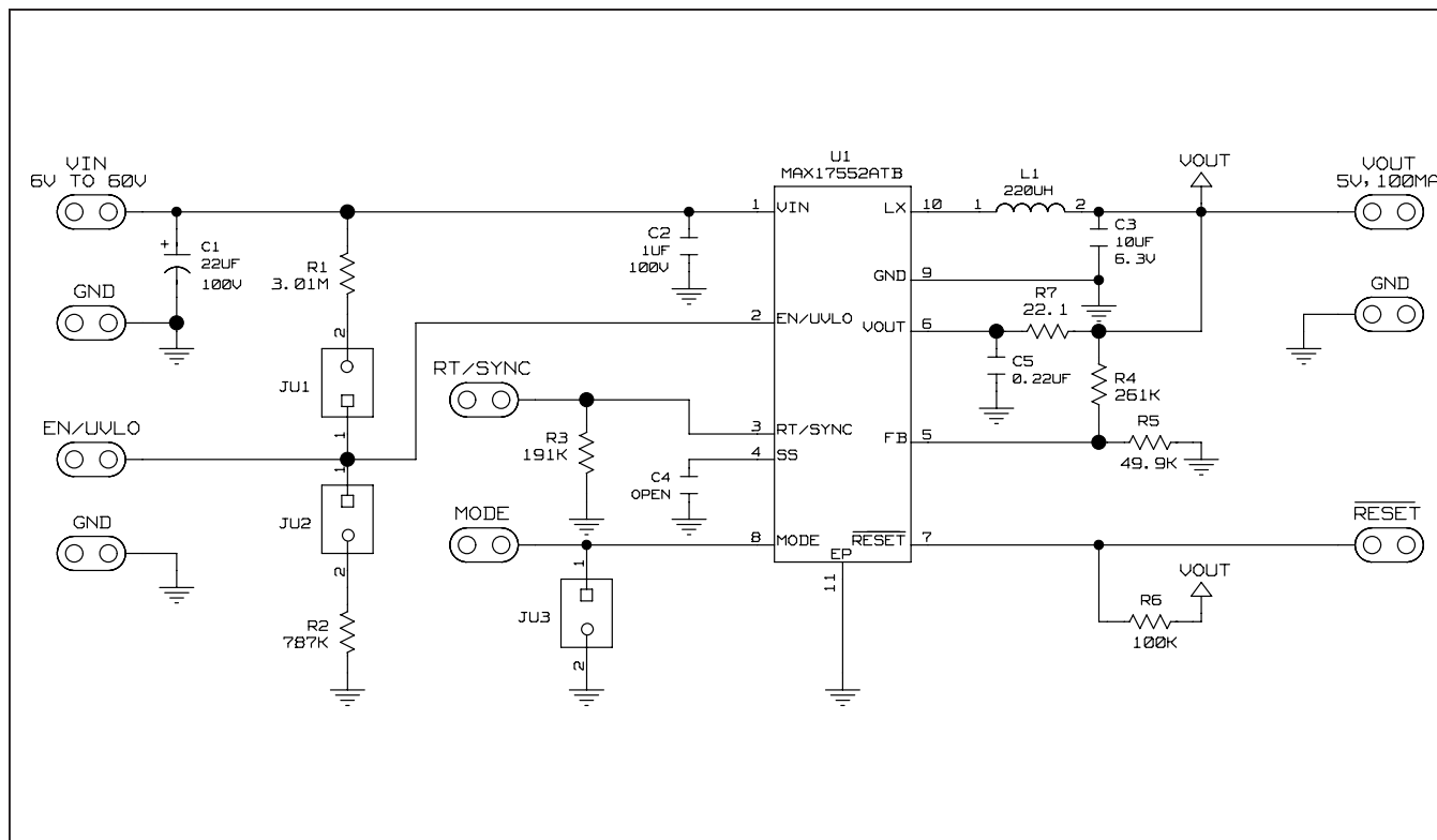
Figure 1. MAX17552 5V EV Kit (TDFN) Schematic
