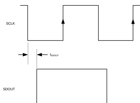
Figure 81. SDOUT Timing
