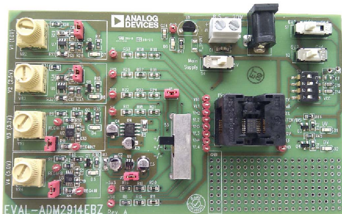
Figure 1. Evaluation Board
