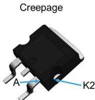
Figure 13. Creepage without top coating
