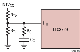
Figure 8. Active Voltage Positioning Applied to the LTC3729
